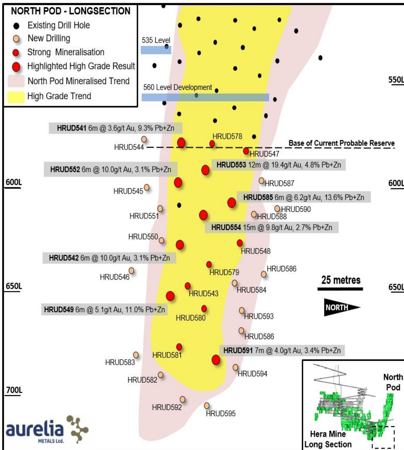
Figure 1. North Pod long section displaying the location of recent drilling results, along with selected intersections. A full list of significant results can be found in Table 2.
