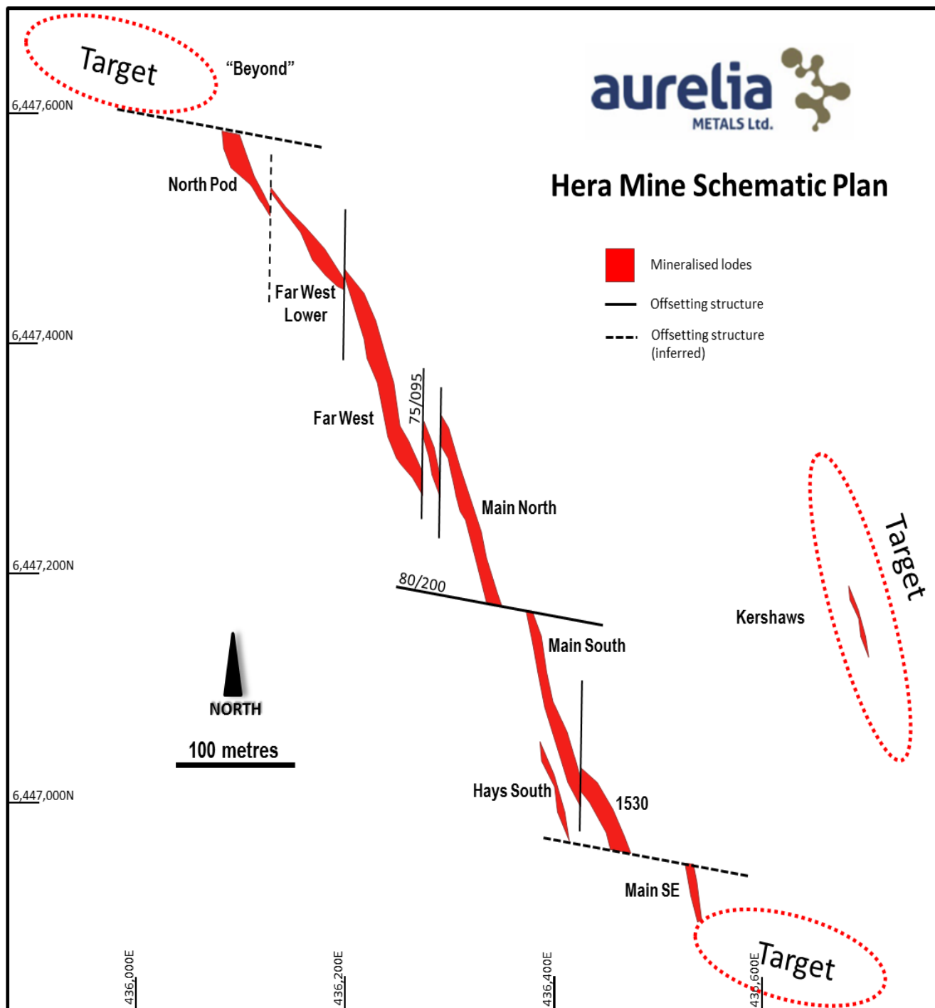
Figure 2. A schematic plan showing the different lodes at Hera, along with the Kershaws prospect to the east.
